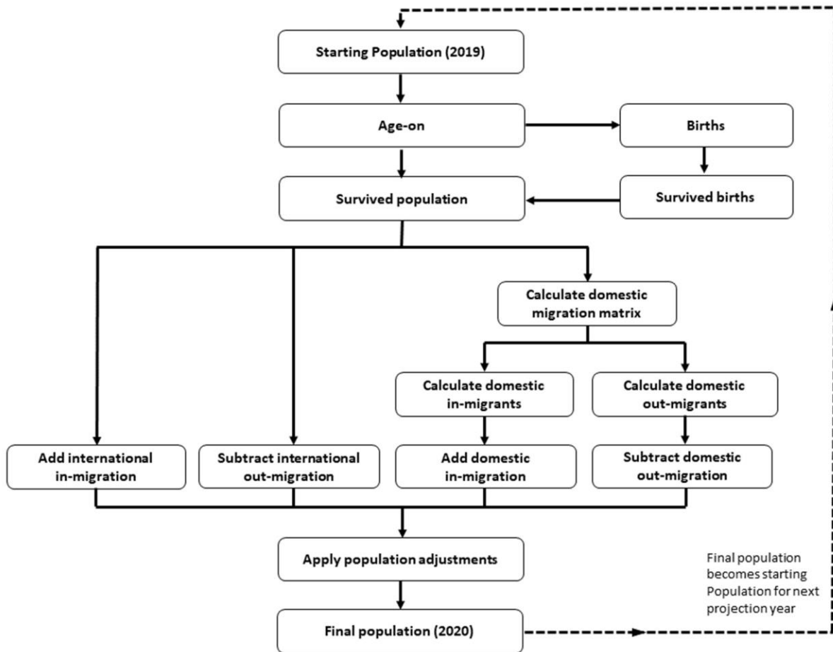
GLA Population Projection: flow chart of the projection cycle
